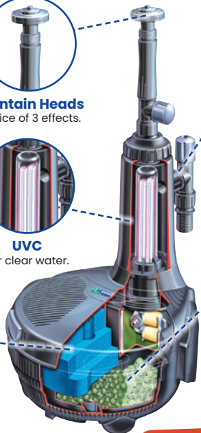
Kaldnes™ Biomedia Great for friendly bacteria.
